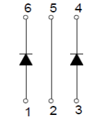
BAT54JW
