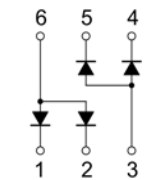
BAT54ADW
