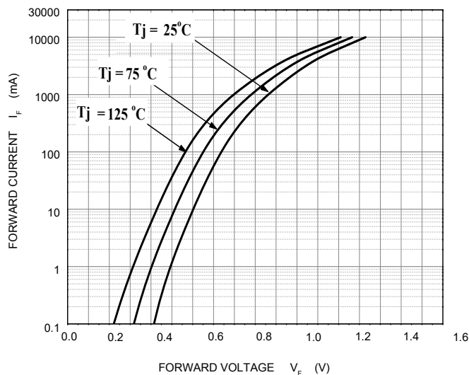
Forward Characteristics
