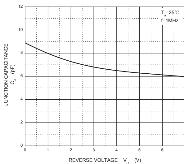
Capacitance Characteristics
